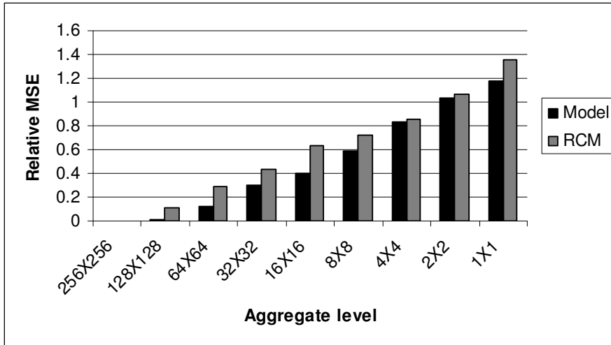
Figure 5.3 Cumulative Relative MSE for homestead at different scales
