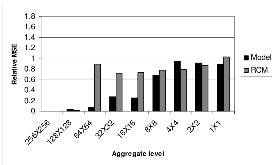
Figure 5.4 Non cumulative Relative MSE for chena at different scales
