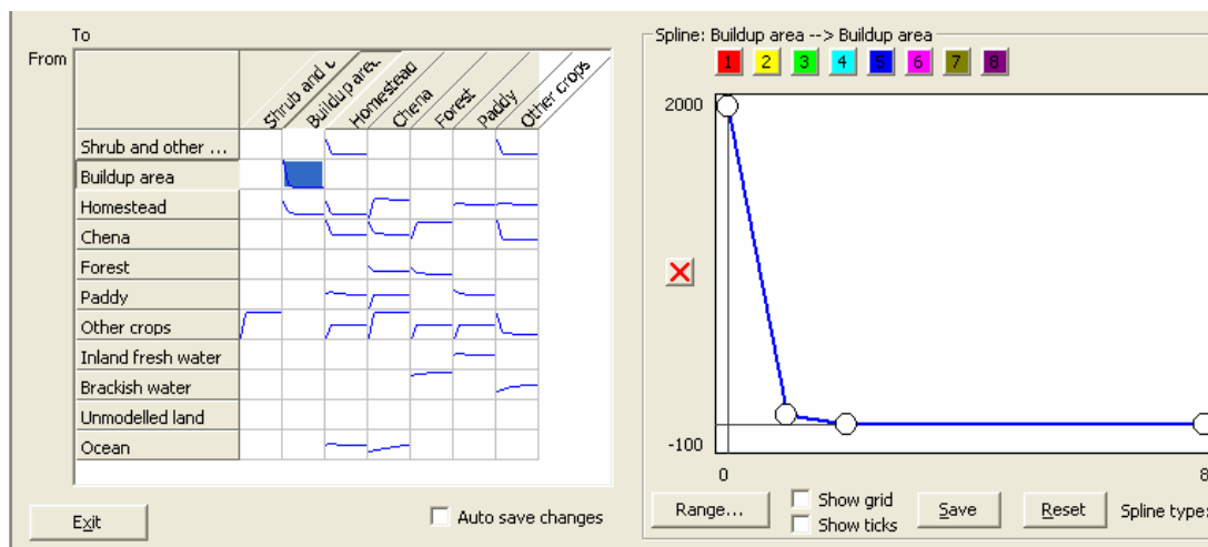
Figure 4.10 The matrix of CA rules
