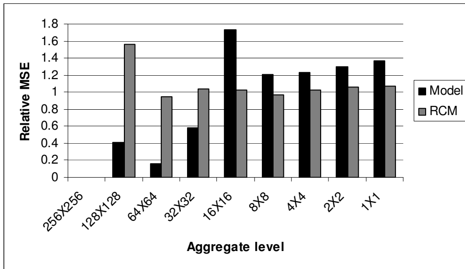
Figure 5.5 Non cumulative Relative MSE for paddy at different scales
