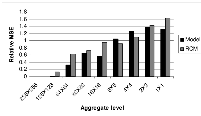
Figure 5.2 Non cumulative Relative MSE for homestead at different scales
